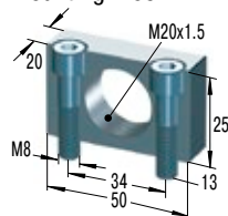
MB20SC2 Mounting Block
