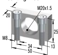
MB20SC2-V4A Mounting Block
