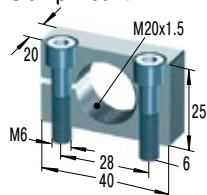
MB20 Clamp Mount
